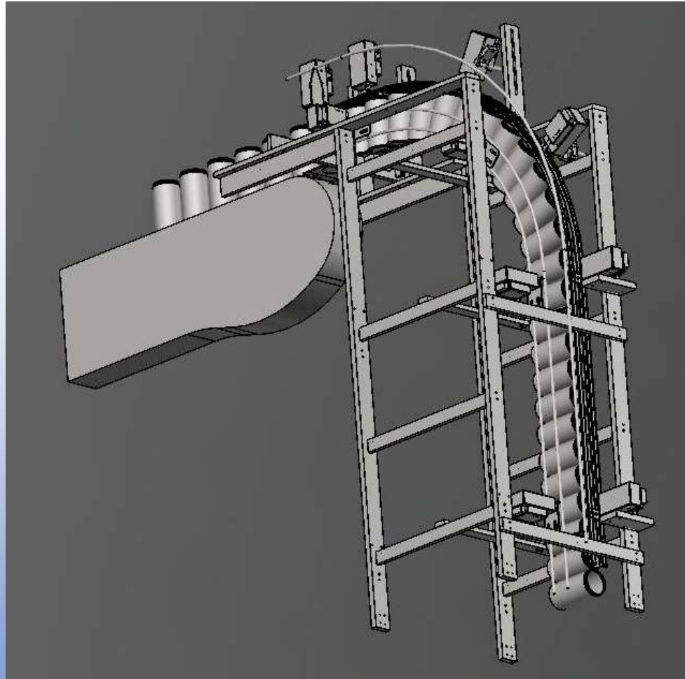
Canister Chute with Side and Top Guide rail adjustment
